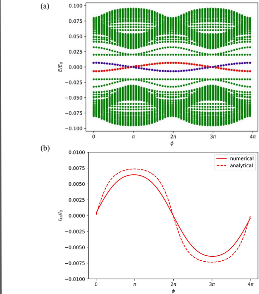
Fig 5. (a) Energy eigenvalues as a function of phase difference between the superconductors, for a TRS broken phase. The states around zero energy show \pi crossing characteristic of MZMs (b) 4\pi periodic current of the corresponding low energy states, also compared with the analytical current obtained from our effective low energy theory in the presence of TRS broken parameter. Numerical calculations performed using Kwant 2 and Hybrid Kernel Polynomial Method 3 .
